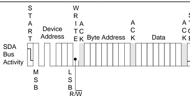
Figure 6. Byte Write
