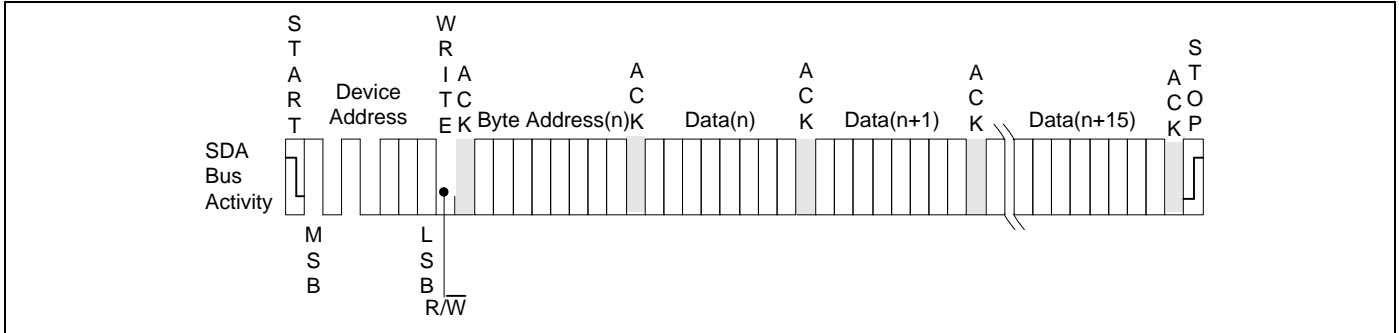
Figure 7. Page Write
