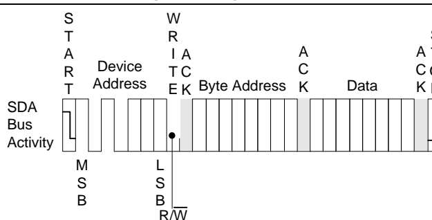
Figure 8. Byte Write
