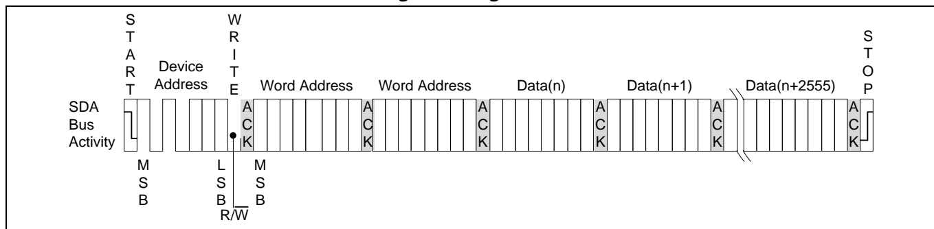
Figure 7. Page Write
