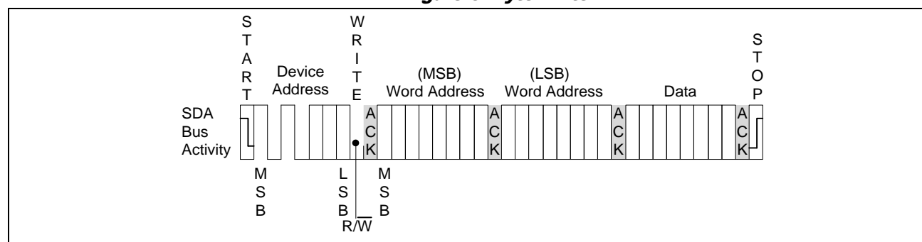
Figure 6. Byte Write
