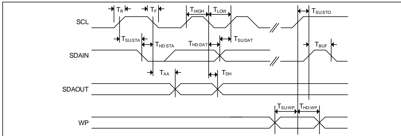
Figure 11. Bus Timing
